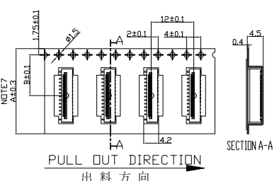
宽度: 16mm/24mm 载带
