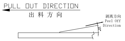
载带上下带剥离强度: 0.1N--1.3N(10g-130g) Peeling off force of top tape: 0.1N--1.3N(10g-130g)
