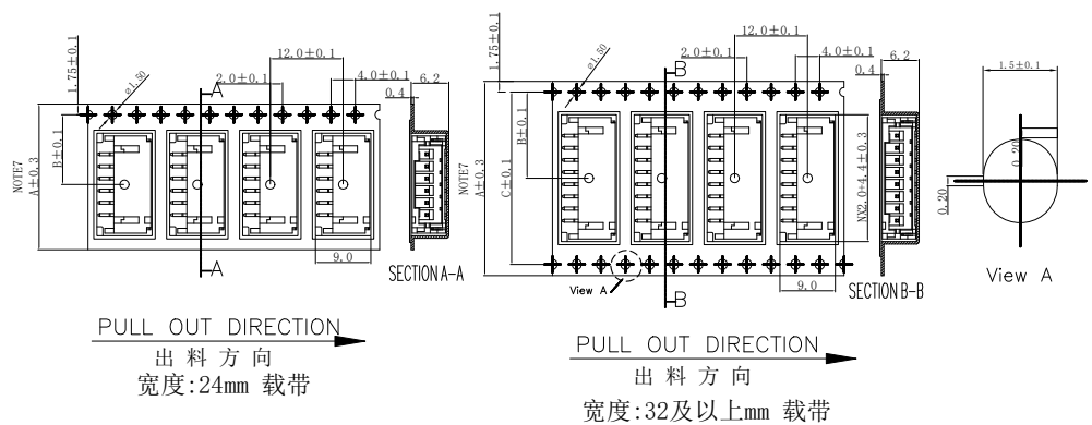
载带上下带剥离强度: 0.1N--1.3N(10g-130g) Peeling off force of top tape: 0.1N--1.3N(10g-130g)
