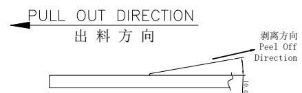
载带上下带剥离强度: 0.1N--1.3N(10g-130g) Peeling off force of top tape: 0.1N--1.3N(10g-130g)
