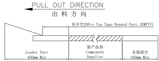
载带带头及带尾尺寸 Lead tape length
